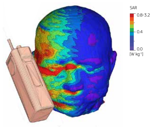
Figure C6 — The specific energy absorption rate (SAR) distribution in the head from exposure to a 380 MHz TETRA (Terrestrial Trunked Radio) handset
