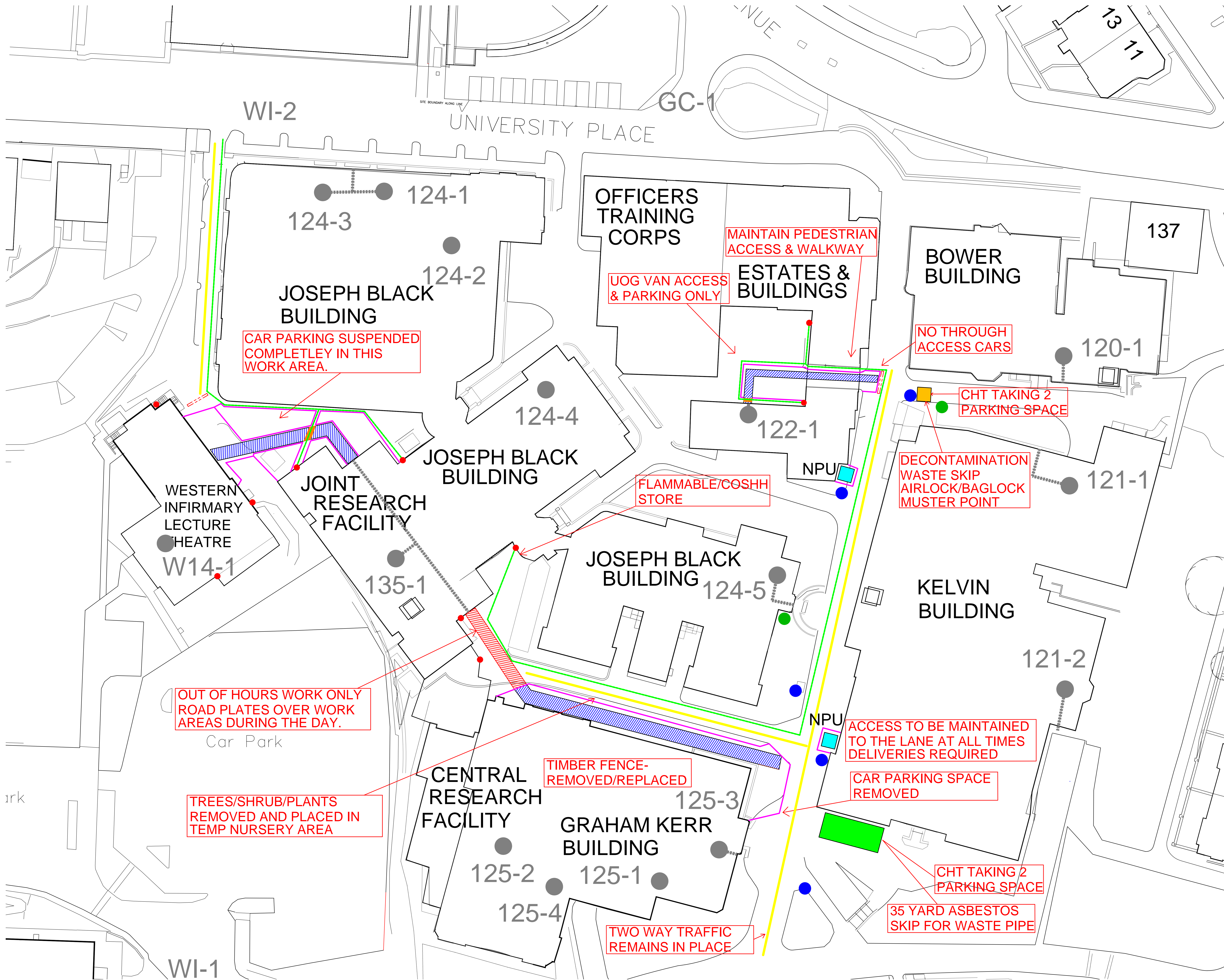
Site Key Plan
