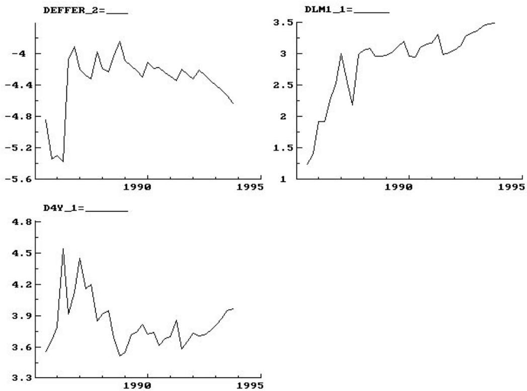
Figure 8(b) Recursive Estimates for New Zealand - t-ratios of Estimated Coefficients
