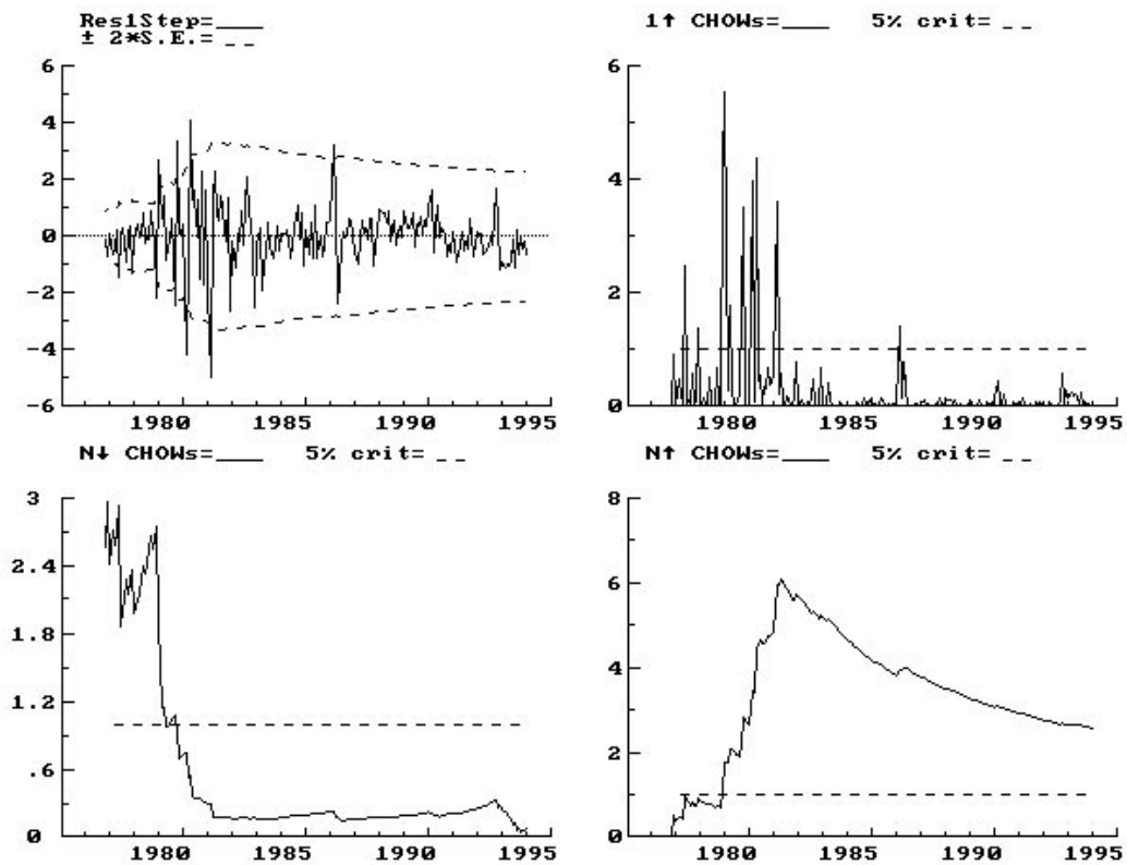
Figure 7(c) - Canada: Recursive Residuals and Chow Tests
