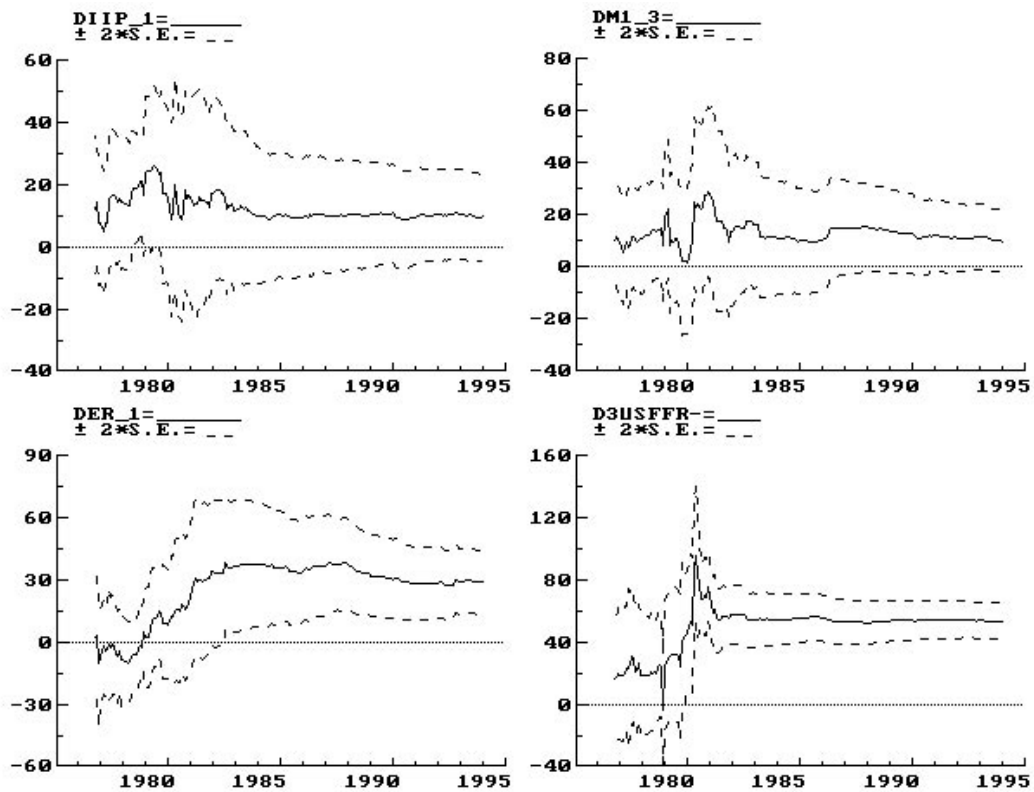
Figure 7(a) Recursive Estimates for Canada - Estimated Coefficients
