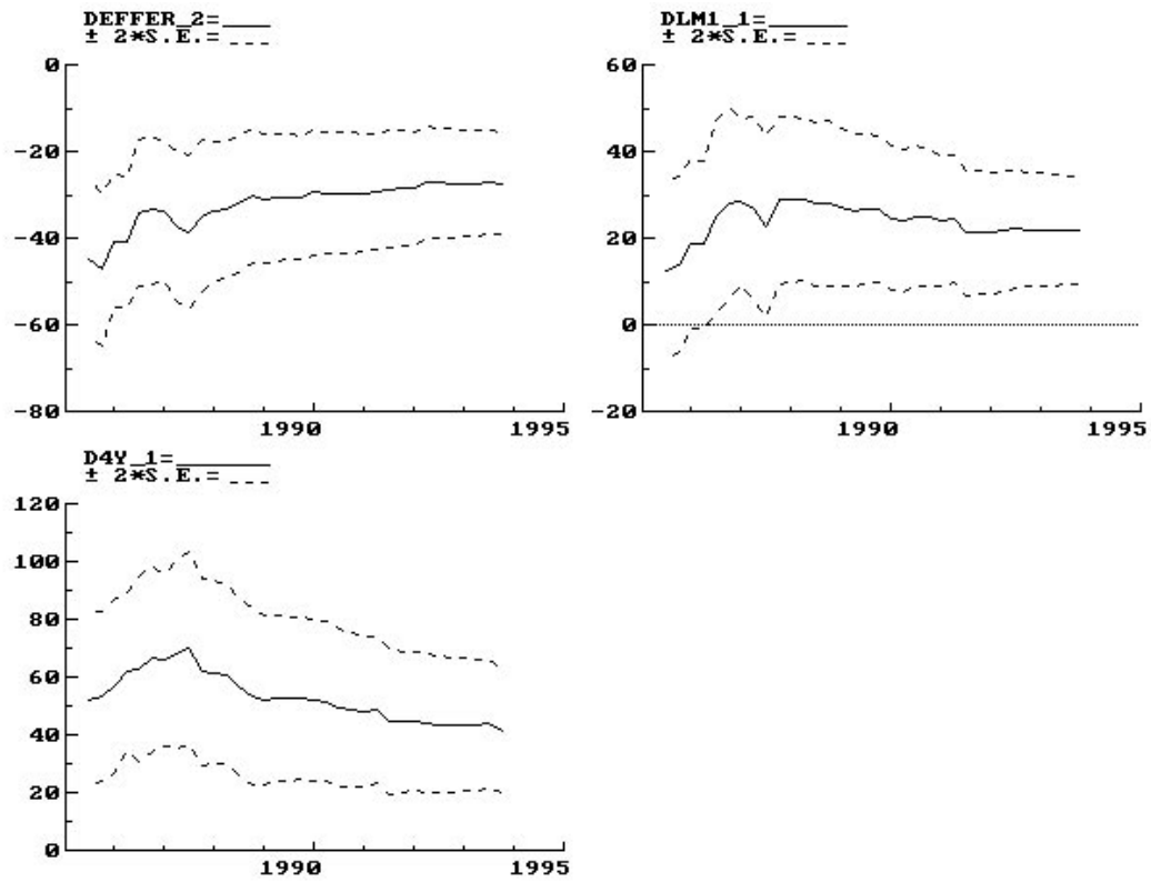
Figure 8(a) Recursive Estimates for New Zealand - Estimated Coefficients
