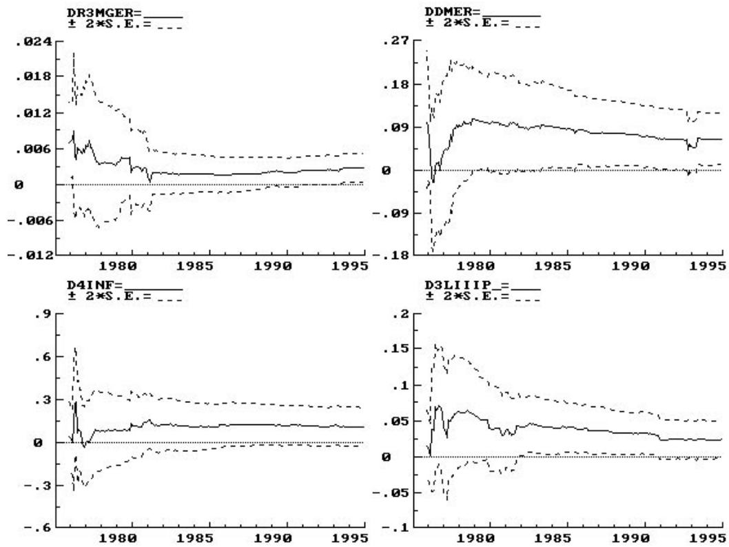
Figure 6(a) Recursive Estimates for Italy - Estimated Coefficients
