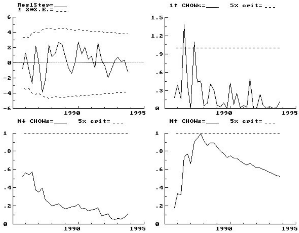
Figure 8(c) - New Zealand: Recursive Residuals and Chow Tests
