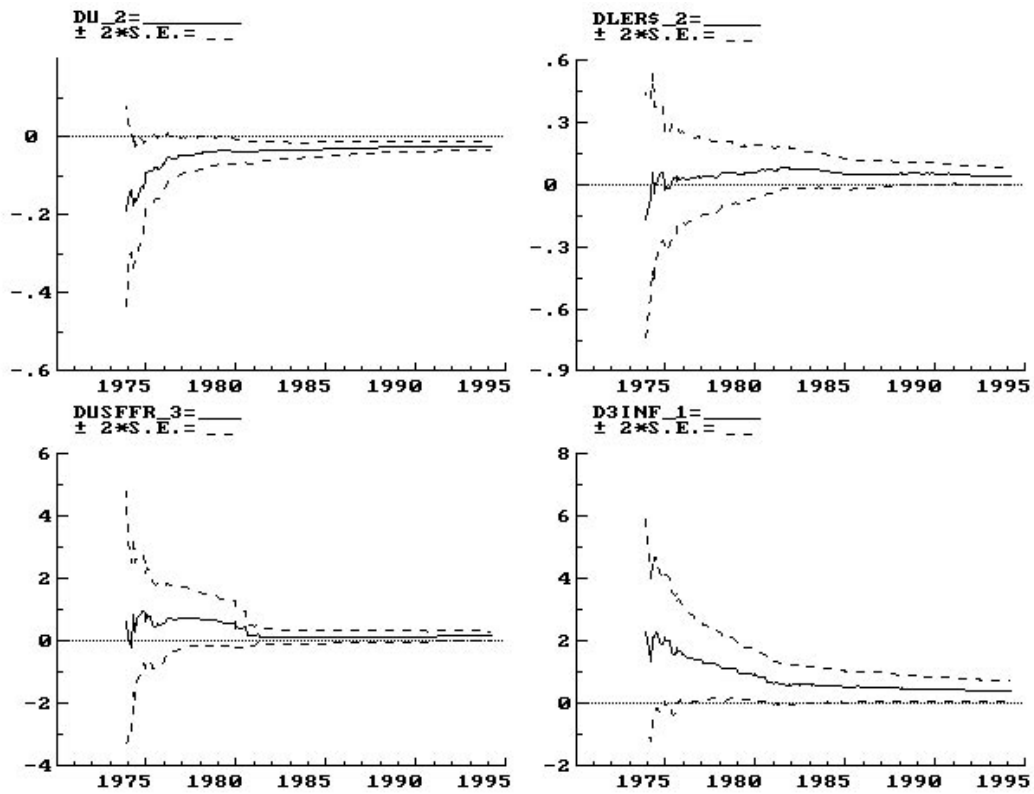
Figure 2(a) Recursive Estimates for Germany - Estimated Coefficients
