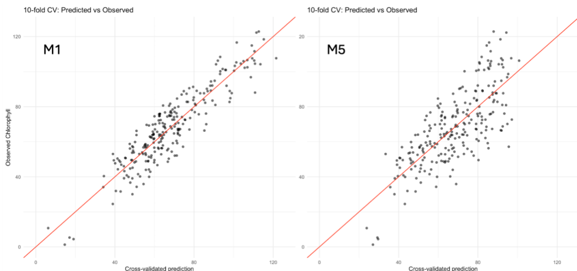
Figure 23.1. A comparison of the predicted and observed values for the out of sample fold from 10-fold cross validation for a quite good predictive model (M1) and a poorer one (M5).
