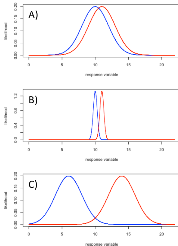
Figure 24.1. Effects of variance and effect size on the ability to detect differences between distributions. A) Small effect size (the difference between the averages of the red and blue distributions) and larger standard deviation means a lot of data would be required to distinguish between the blue and red distributions. B) The averages are the same as A, but a smaller standard deviation would make the two distributions easier to distinguish from each other. C) Increasing the effect size means that even with large standard deviations, differences could be distinguished, even without enormous sample sizes.
