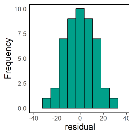
Figure 7.2. The frequency histogram of residuals from the data and model shown in Fig. 7.1.
