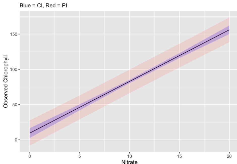
Figure 23.3. A comparison of the confidence interval (purple) for the regression line (black) and the prediction interval (pink).
