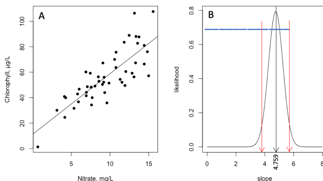
Figure 20.1. A) The relationship between Chlorophyll and Nitrate, and B) the distribution of the estimated slope. The blue lines indicate the width of the standard deviation (0.503) of the estimated mean (4.759), showing that there are more than 9 standard deviations 'between' the mean and zero; and the red lines indicate the position of the 95% confidence interval: 3.746 – 5.772, (see section 20.3 ).
