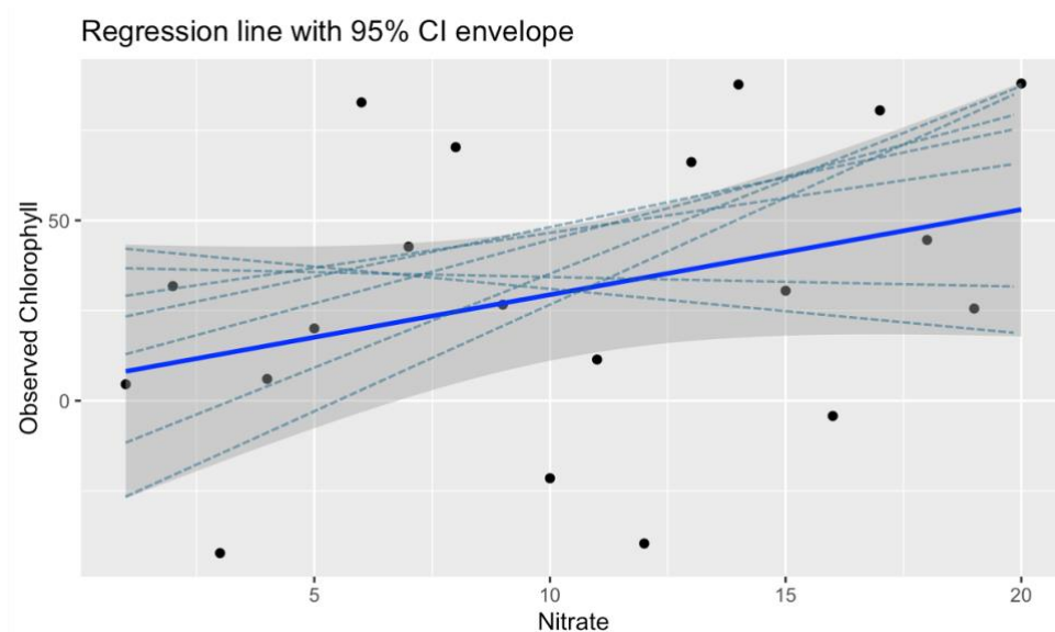
Figure 23.2. An example of a confidence envelope (dark grey) around a regression line (solid blue line). The 95% confidence envelope contains the true regression line
