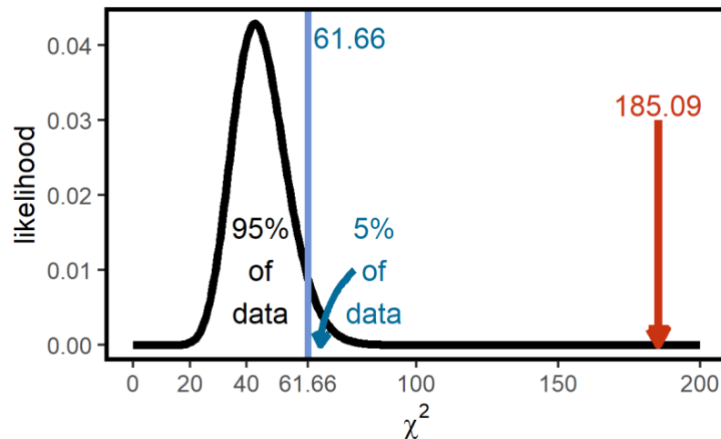
Figure 18.1. A \chi^2 distribution with 45 dfs and the position of the 95 th quantile shown in blue. The area under the curve to the left of the blue line accounts for 95% of the area under the curve. Observed values of the test statistic between 0 and 61.66 would not be regarded as improbable (assuming a threshold p-value of 0.05). Observed values to the right of the blue line would suggest that the residual deviance is not consistent with the null hypothesis that the overdispersion has arisen by chance alone. The p-value that would be routinely cited from this test would be the area under the curve to the right of the red arrow (which is very very small indeed, so p < 0.0001 ).
