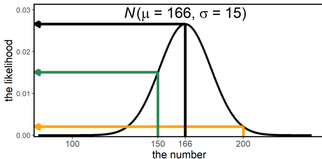
Figure 4.1. A Normal distribution with \mu = 166 and \sigma = 15 , or N(166, 15) . The y-axis indicates how likely we are to encounter a number on the x-axis. So, 100 or 250 are very unlikely (because they are in the tails of the distribution) but the likelihoods of say 200 , 150 , and 166 are increasingly larger.
