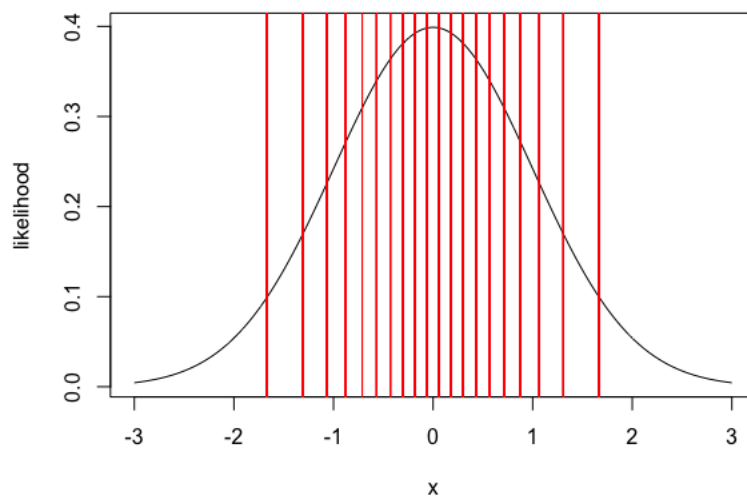
Figure Q.1. 20 quantiles of the Normal distribution. The value of each quantile is where the red line intercepts with the x-axis. Each vertical slice of the distribution is equal in area .
