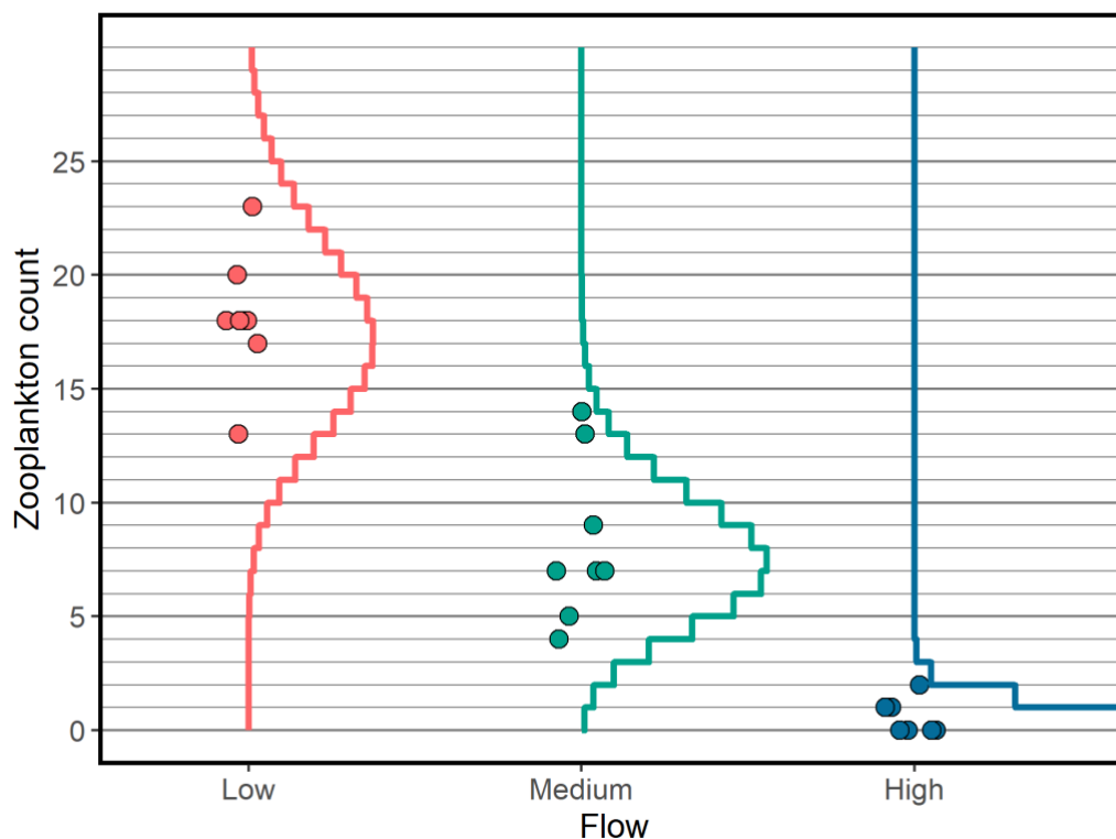
Figure 11.1. Plot of Zooplankton count against Flow rate. Data points are modelled assuming a Poisson distribution whose mean (and variance) are conditioned on the explanatory variables. In this case the explanatory variable is categorical with 3 levels.
