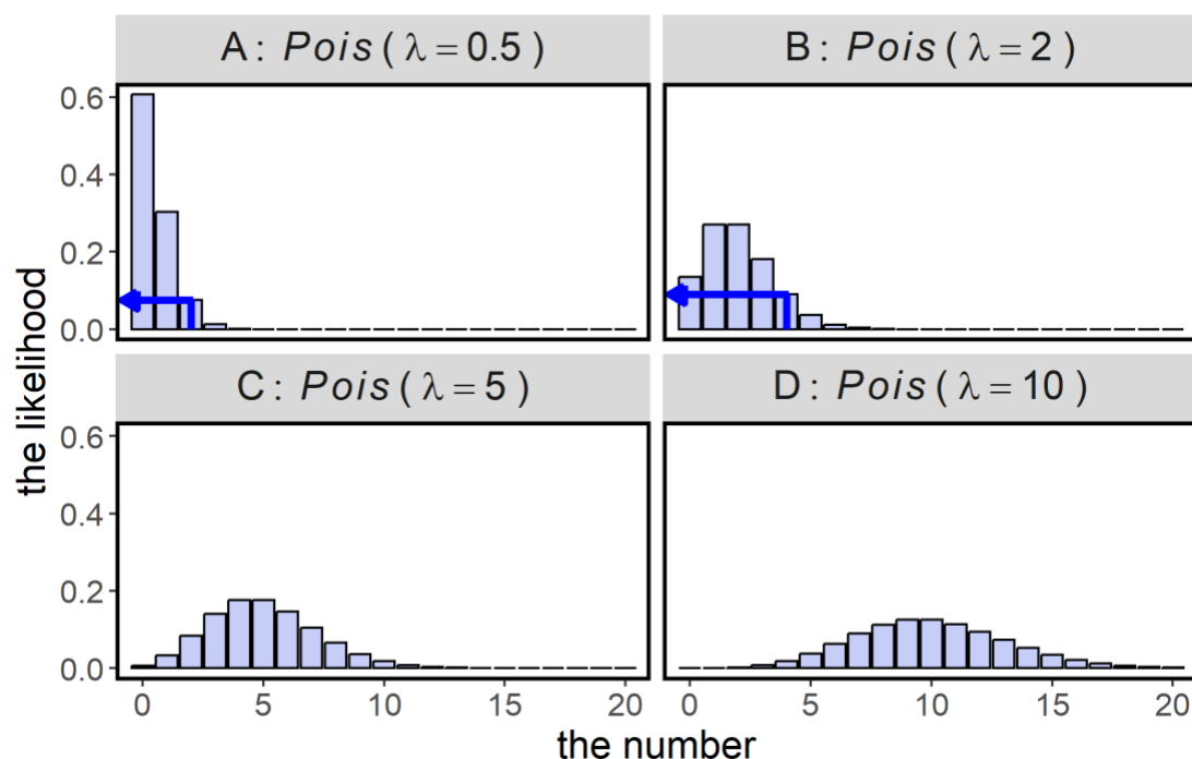
Figure 4.4. Four Poisson distributions with A) \lambda = 0.5 , B) \lambda = 2 , C) \lambda = 5 , D) \lambda = 10 respectively. Because it is a discrete distribution the likelihood (or probability) changes in a step-like way.
