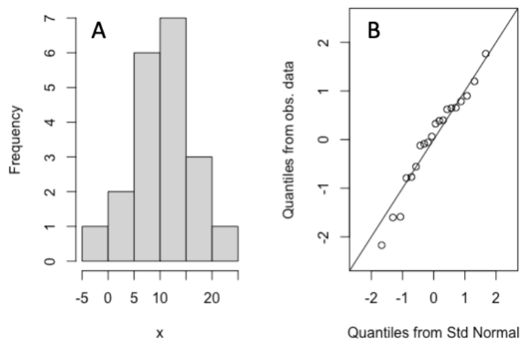
Figure Q.2. A) The original observed data. B) qqplot after standardizing the observed data. The points mostly fall close to the x=y line because the data is close to Normally distributed.
