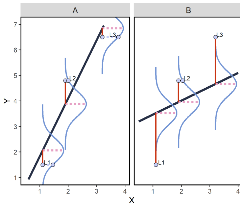
Figure 13.2. Visualizing the likelihood of each data point (blue points) given a model for a best-fitting line (A), and a poorly-fitting line (B). Each point is assumed to derive from (in this example) a Normal distribution whose mean (indicated by the dashed pink line) is predicted from the line (black)
