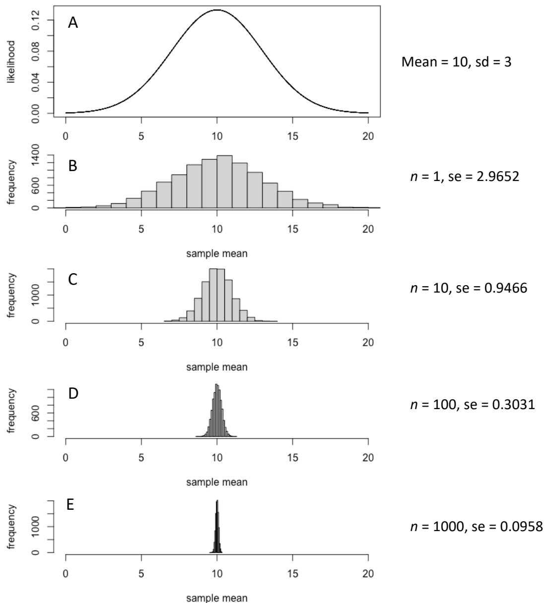
Figure S.1. Demonstration of a shrinking standard error. A: A Normal distribution, mean = 10, standard deviation = 3. Figures B-E show the distribution of the means of samples of different sizes from the distribution in A. B: the mean calculated from just a sample of n = 1 . Unsurprisingly, this is just a manifestation of the parent distribution. C: means computed from a sample size of n = 10 . D: means computed from a sample size of n = 100 . E: means computed from a sample size of n = 1000 . As n increases, the means of each sample become increasingly stable and closer to the mean of the parent distribution, resulting in reduction of the standard error (or standard deviation of the mean). The standard error of distributions in B – E is the standard deviation of the sample divided by the square root of n : s/\sqrt{n} .
